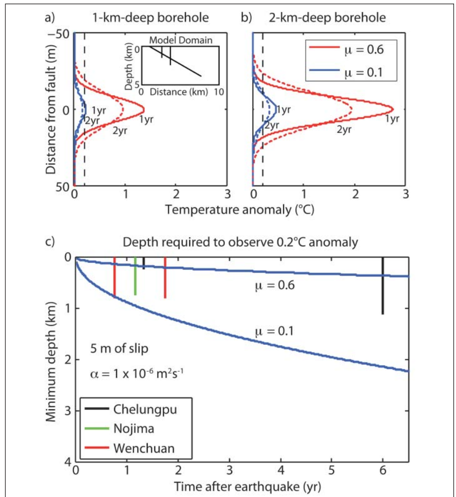
Fig. 1. Modeled frictional temperature anomalies resulting from a thrust earthquake with 5 meters of slip assuming a thermal diffusivity ( \alpha ) of 10^{-6} square meters per second. (a) Temperature anomaly for a borehole intersecting the fault at a depth of 1 kilometer. Red and blue curves show frictional heating for effective friction coefficients ( \mu ) of 0.6 and 0.1, representing a strong and weak fault, respectively. Solid and dashed curves show the frictional heating anomaly 1 and 2 years, respectively, after the earthquake. Dashed black line shows the assumed detection threshold of 0.2^\circ\text{C} ; temperatures lower than this value cannot firmly be attributed to fault processes. (b) Temperature anomaly for a borehole intersecting the fault at 2-kilometer depth. Note how the deeper boreholes allow scientists to see a clearer temperature signal in both types of faults. (c) Blue curves show the minimum depth of borehole intersection with a fault to observe a temperature anomaly of 0.2^\circ\text{C} as a function of time. The depth and timing of borehole completion of fault zone drilling experiments are shown as vertical lines at the top of the plot. Calculations and plots are from Fulton et al. [2010].
