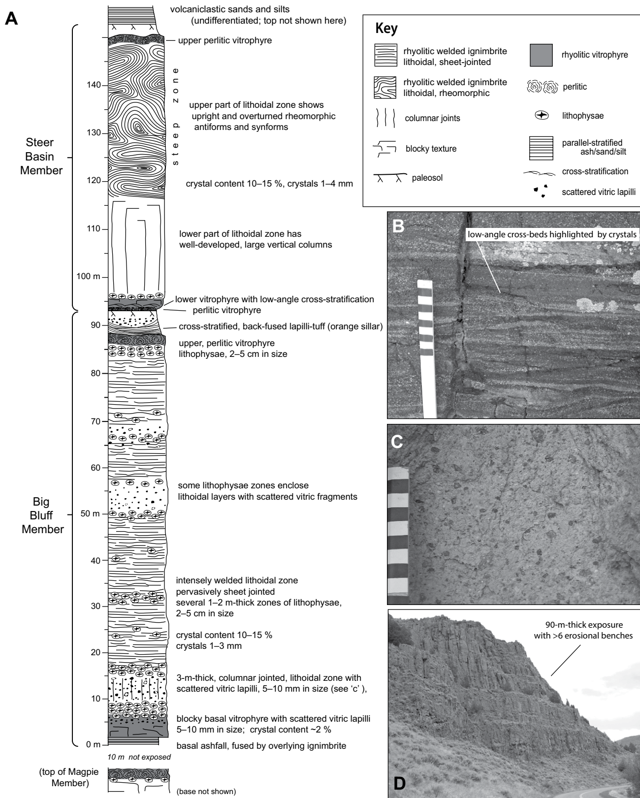
Figure 5. (A) Big Bluff and Steer Basin Members, at Maggie Basin (42°15'01.3"N, 114°15'51.2"W). (B) Low-angle cross-stratification highlighted by crystals in the lower vitrophyre of the Steer Basin Member. (C) Abundant scattered angular vitric fragments supported in tuff matrix in the lower lithoidal zone of the Big Bluff Member. (D) Big Bluff Member in Rock Creek Canyon: Benches mark successive lithophysal zones showing the compound nature of the ignimbrite.
